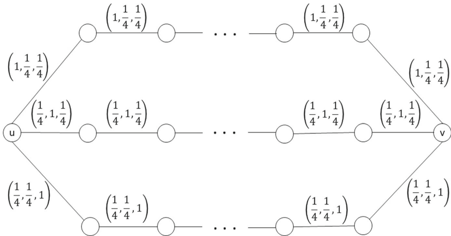
Fig. 1 An illustration of our lower bound construction for t = 3
